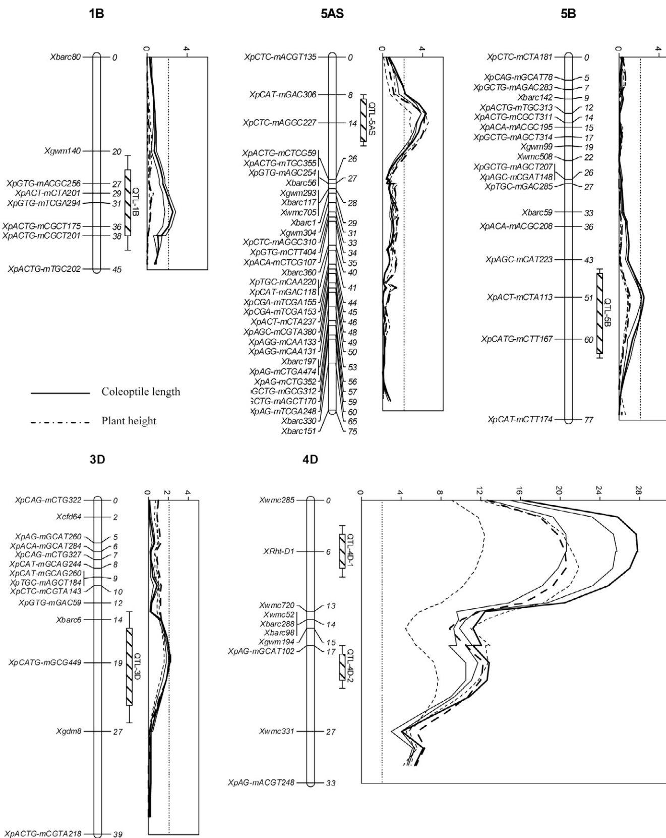
Figure 2. Log likelihood ratio (LOD) contours obtained from interval mapping of the Wangshuibai × Wheaton population that show quantitative trait loci (QTL) locations for wheat ( Triticum aestivum L.) coleoptile length and plant height traits. Bars indicate QTL locations, and bar lengths represent 1-LOD support intervals.
